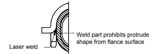
SECTION C-C SCALE 2:1
