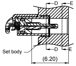
RECOMMENDED SET BODY SIDE HOLE SHAPE
