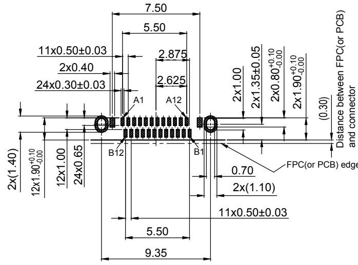
RECOMMENDED PCB LAYOUT DEFAULT TOLERANCE: ±0.05
